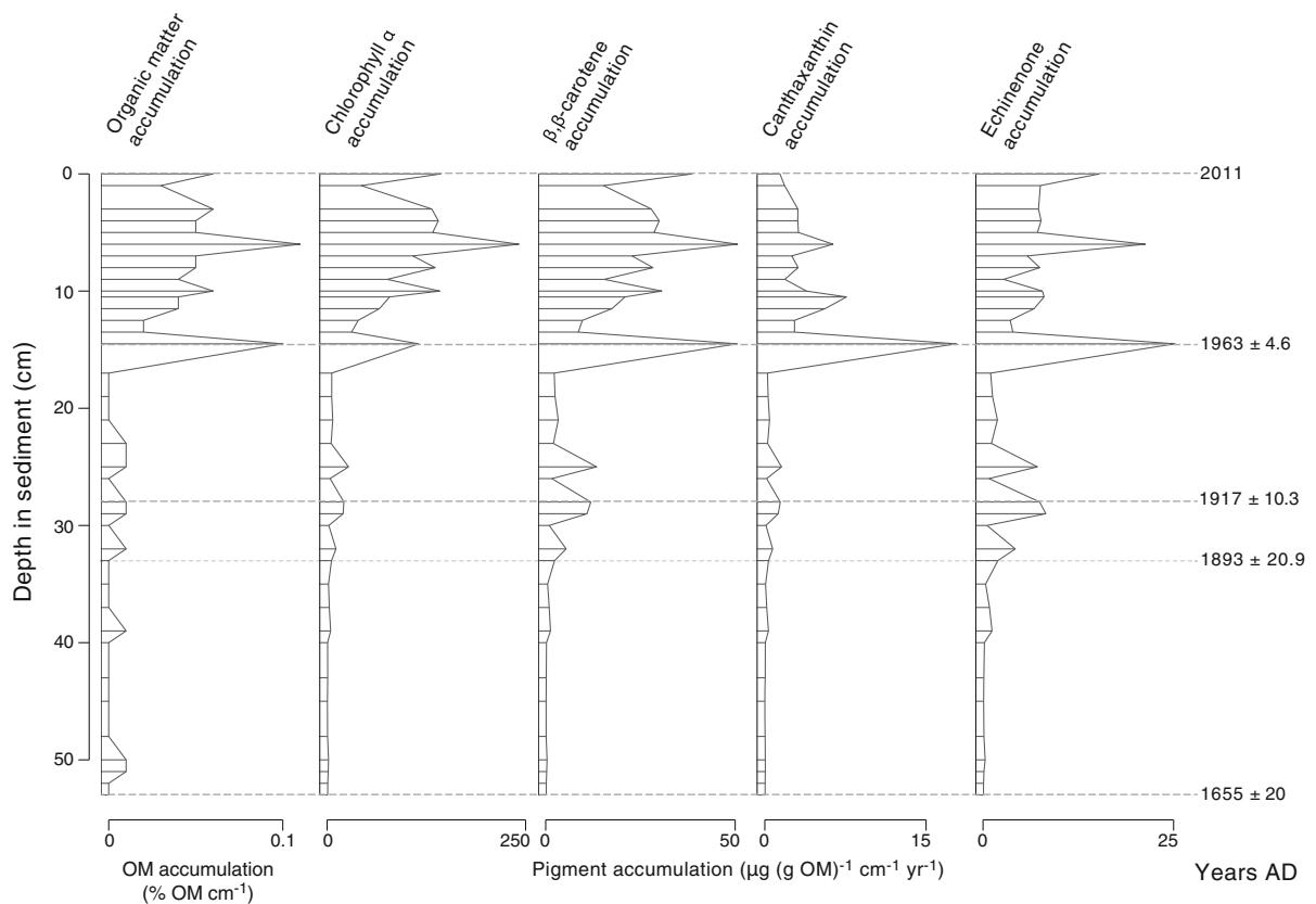
Fig. 5 Stratigraphic plot of organic matter and pigment accumulation rates
